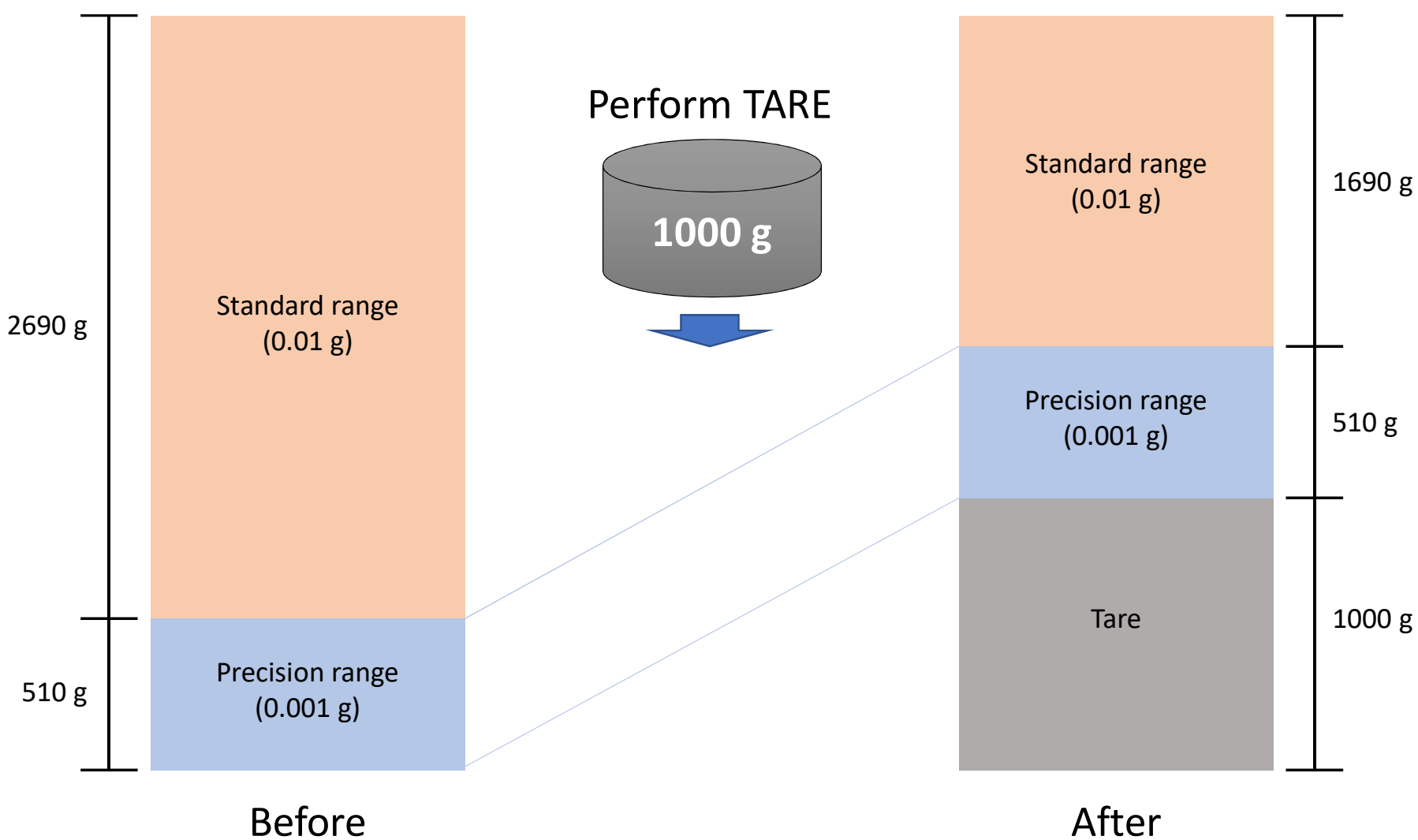
Precision range (0.001 g) of the AD-4212C-3100 before/after performing tare
